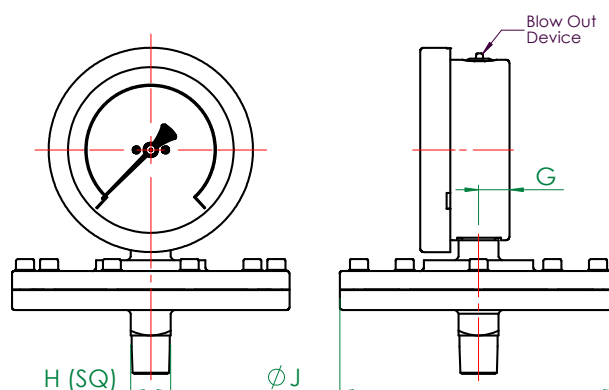
MODEL - 2012 Threaded Connection RANGE - 40 - 400 mbar
