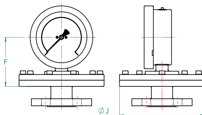
MODEL - 2013/F Flanged Connection RANGE - 40 - 400 mbar
